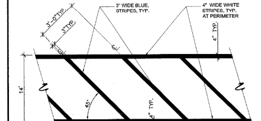
ADA CROSS STRIPPING NO SCALE 7
