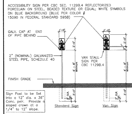
ADA SIGN MOUNT. HEIGHT NO SCALE 6
