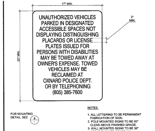
TOW-AWAY SIGN NO SCALE 5
